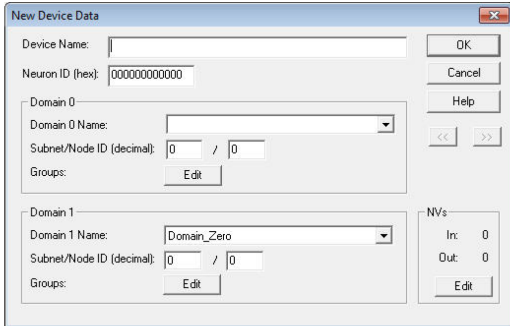
Figure 28. New Device Data Dialog
