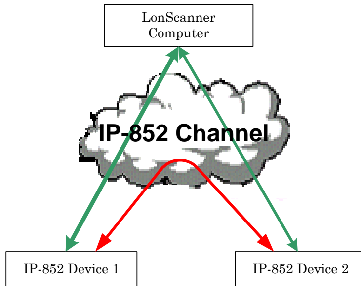
Figure 7. Using LonScanner to Monitor an IP-852 Channel
