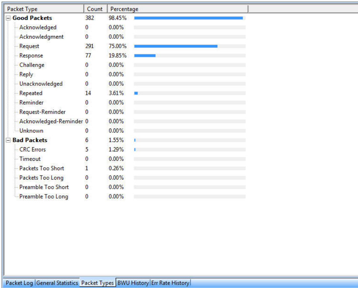
Figure 13. Packet Types Tab
