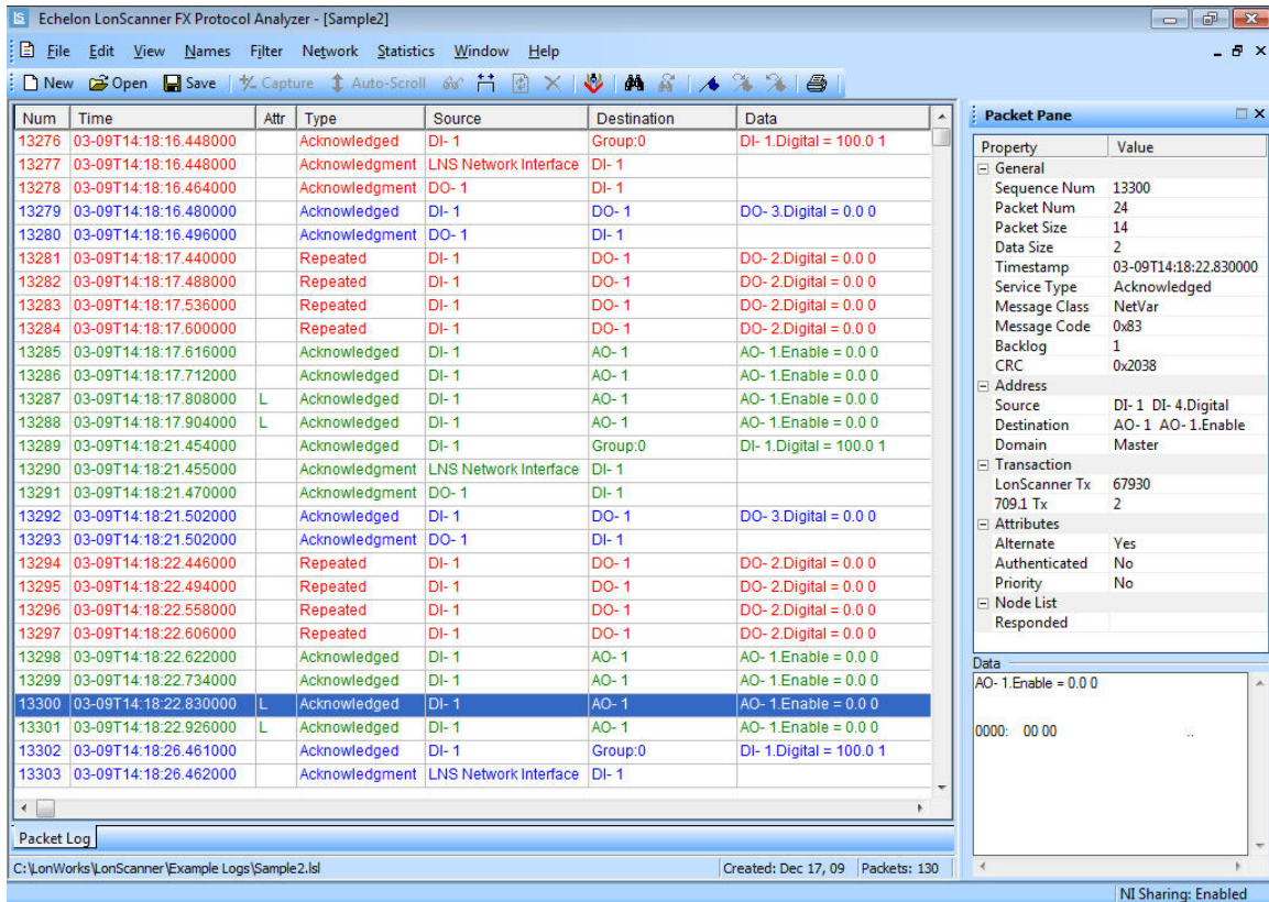
Figure 45. Example Log File Two – Packet 24 Selected
