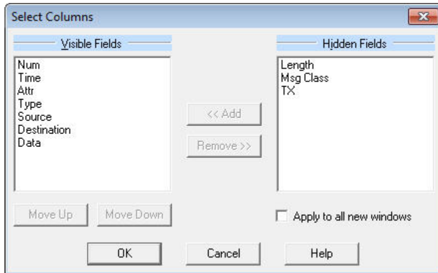
Figure 37. Select Columns Dialog
