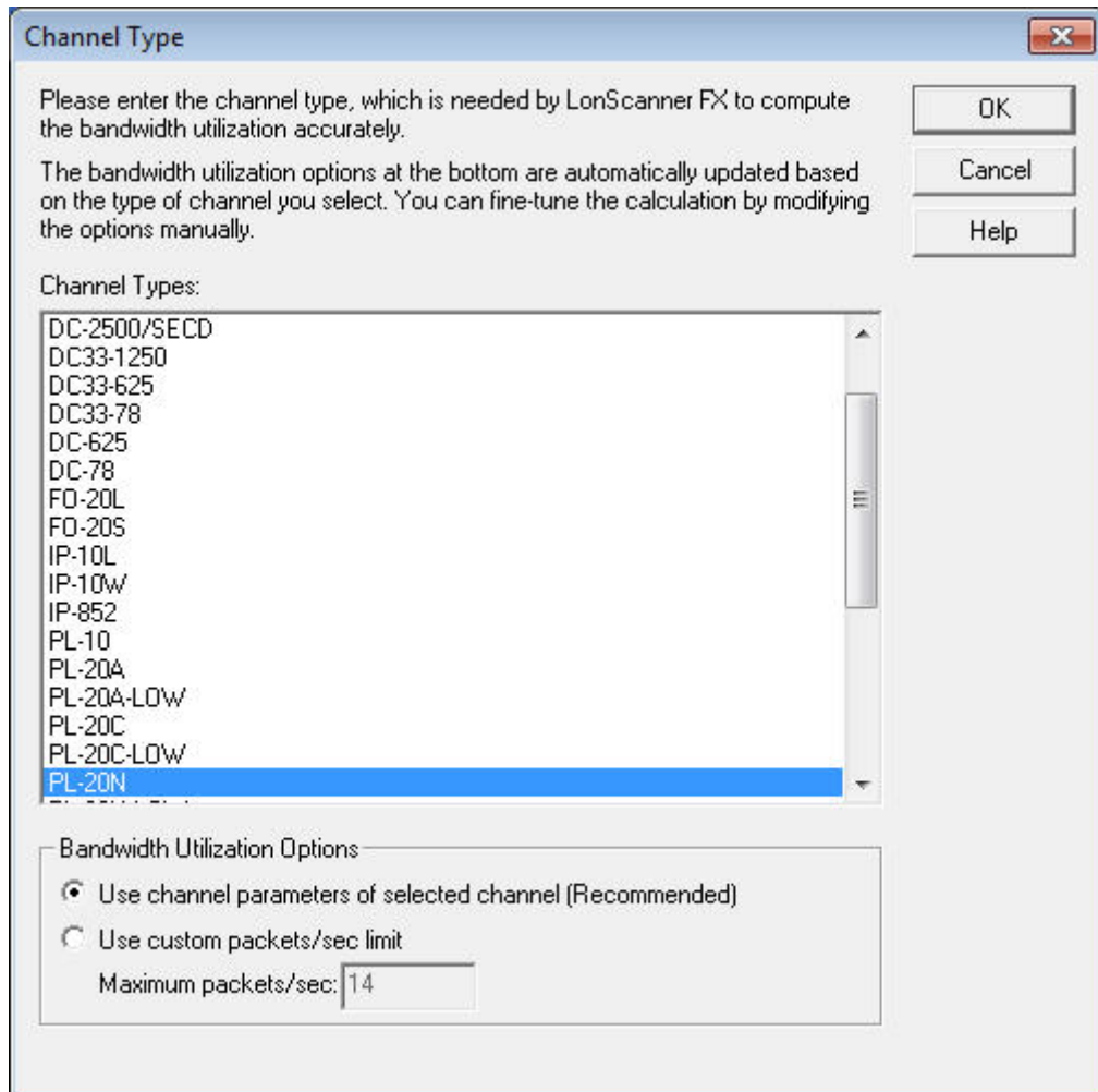
Figure 19. Channel Type Dialog
