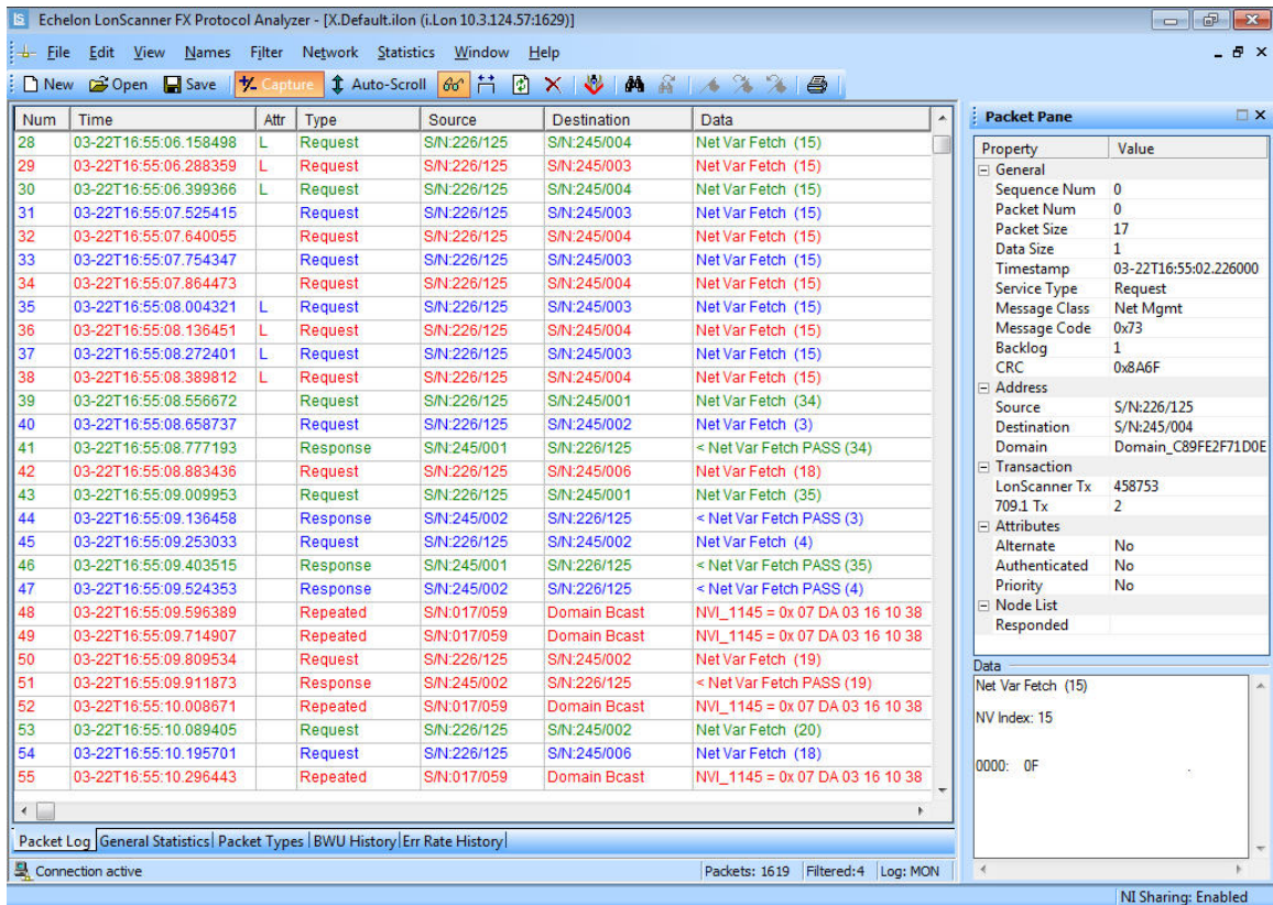
Figure 5. Main LonScanner Window
